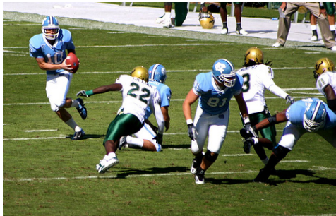
predicted
