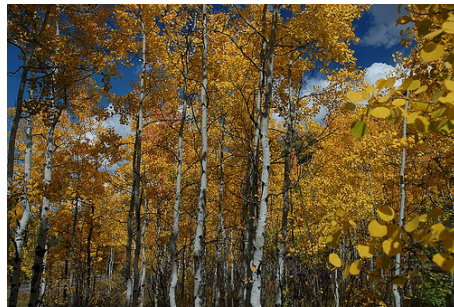
random control
