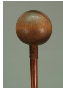
random control
