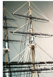
random control
