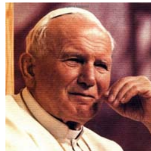
random control
