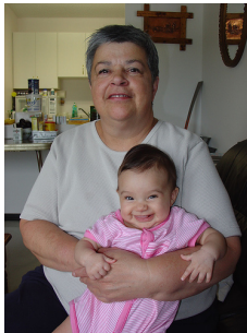
predicted
