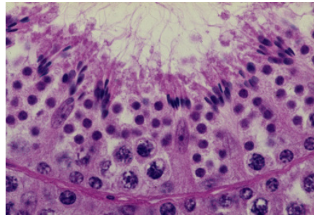
random control
