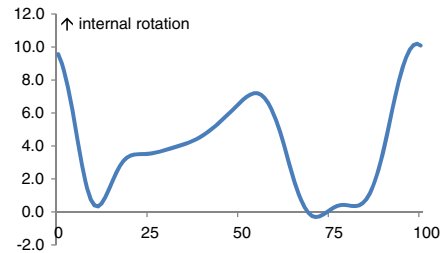
Rearfoot transverse plane motion relative to tibia (°)
