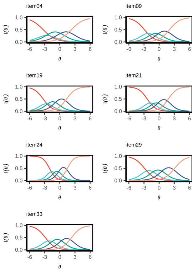
Fig. S1 Option Characteristics curve (Continued)
