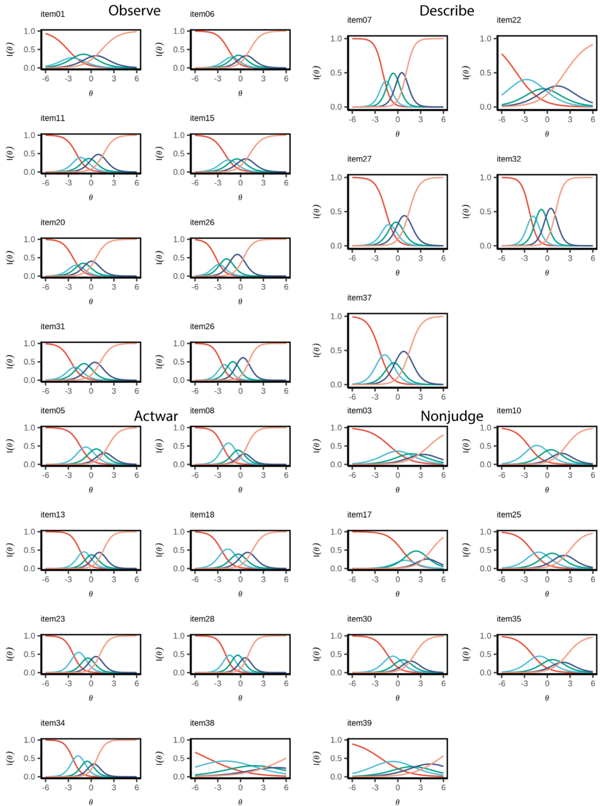
S.Fig.1 Option Characteristics curve
