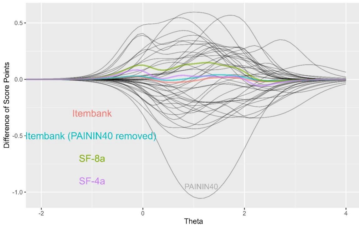
Figure S2 illustrates the difference of expected test scores between thetas based on the U.S. item parameters and thetas based on the German item parameters. Each black line represents a single item of the item bank. Colored lines represent combinations of items.
