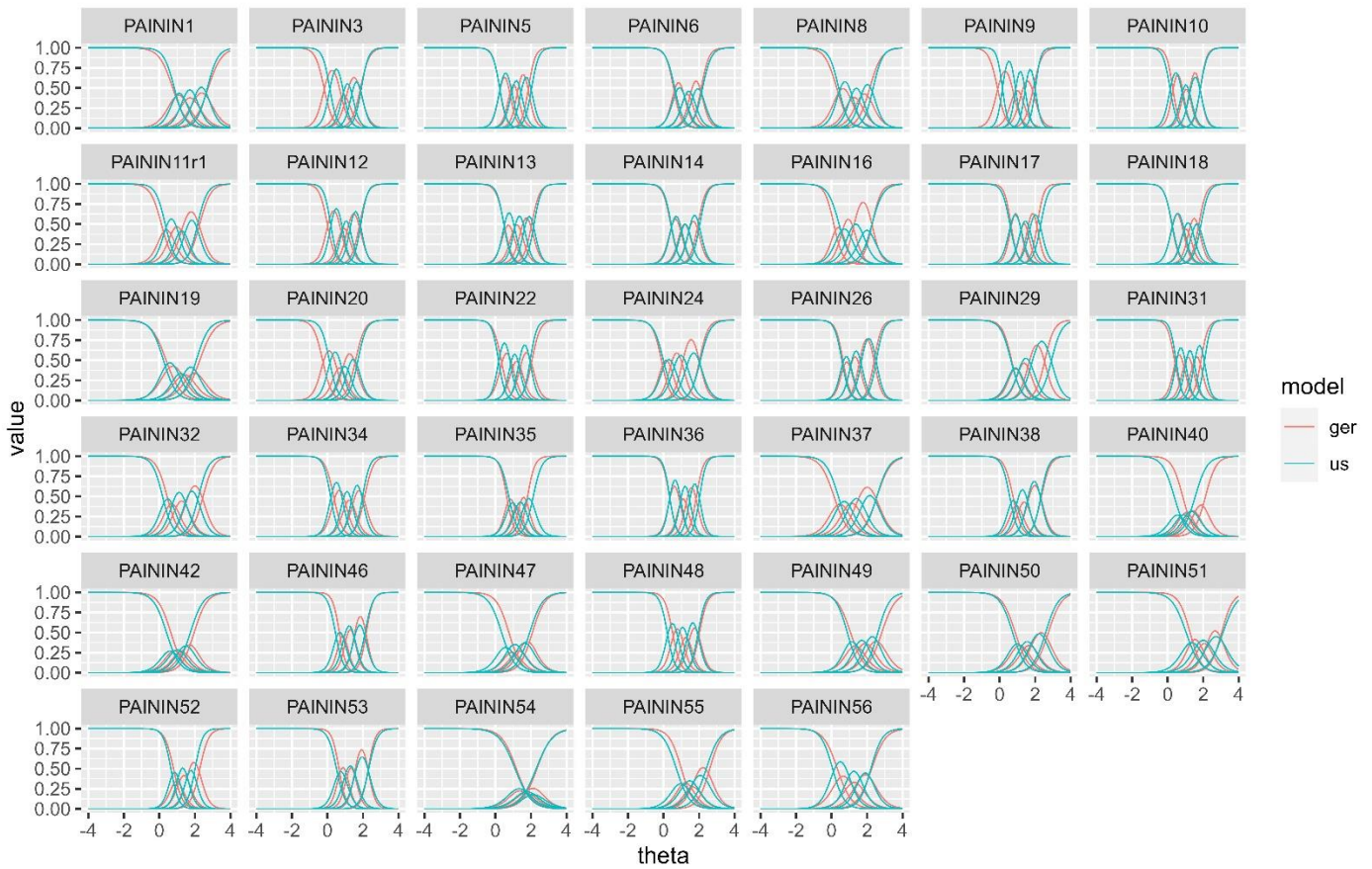
Figure S1 illustrates the item characteristic curves (ICCs) for each of the 40 PROMIS pain interference items. The green curves represent the original U.S. parameters, and the red curves represent the newly estimated parameters based on a German sample.
